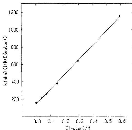
Figure 6. The effect of water on the rate of decomposition of 1^{\bullet-} . The k_{\text{obs}} were calculated assuming the \text{eCe}_h mechanism.
