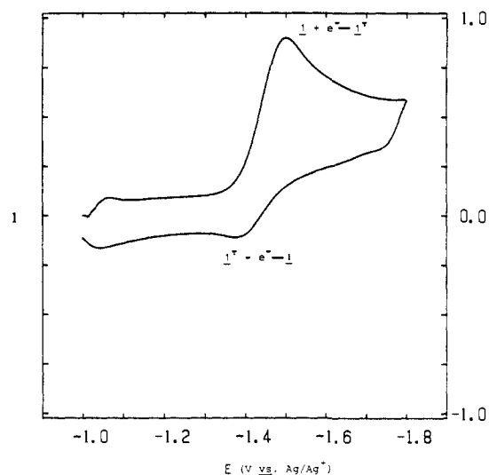
Figure 2. Cyclic voltammogram for the reduction of 1 (1.0 mM) in \text{CH}_3\text{CN}/\text{Et}_4\text{NBF}_4 (0.1 M) at 293 K and 100 V/s.
