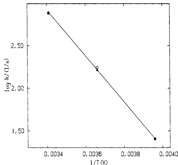
Figure 4. Arrhenius plot for the reactions of 1^{\cdot-} in \text{CH}_3\text{CN} (*) and \text{CD}_3\text{CN} (O) containing \text{Et}_4\text{NBF}_4 (0.1 M).
