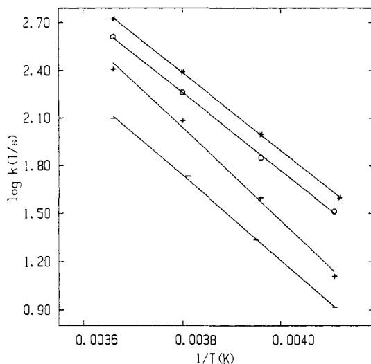
Figure 5. Arrhenius plots for the reactions of diazocarbonyl anion radicals: (*) 5^{\ominus} in \text{CH}_3\text{CN}/\text{Et}_4\text{NBF}_4 (0.1 M), (O) 5^{\ominus} in \text{DMF}/\text{Et}_4\text{NBF}_4 (0.1 M), (+) 1^{\ominus} in \text{CH}_3\text{CN}/\text{Et}_4\text{NBF}_4 (0.1 M), and (-) 1^{\ominus} in \text{DMF}/\text{Et}_4\text{NBF}_4 (0.1 M).
